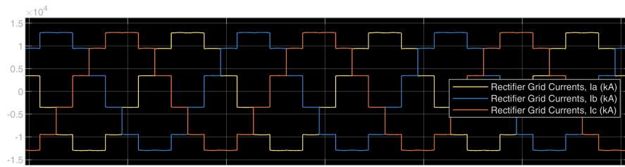
Figure 9: Rectifier AC Grid Currents
