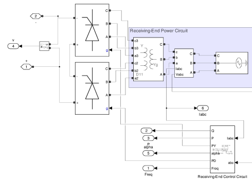
(b) Receiving Power Circuit:
