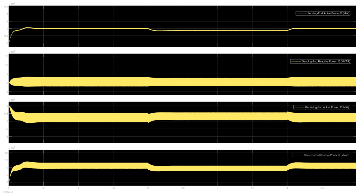
Figure 14: Powers Scope: Shows the resulting active and reactive power transfer limitations dictated by the severe voltage sag on the sending end.
