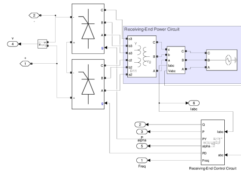
(b) Receiving Power Circuit: Transformer and bridges.
