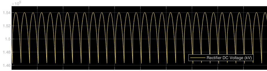
Figure 15: Rectifier DC Voltage ( V_{rect} )
