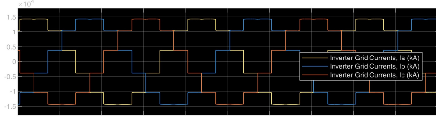
Figure 21: Inverter Grid Currents
