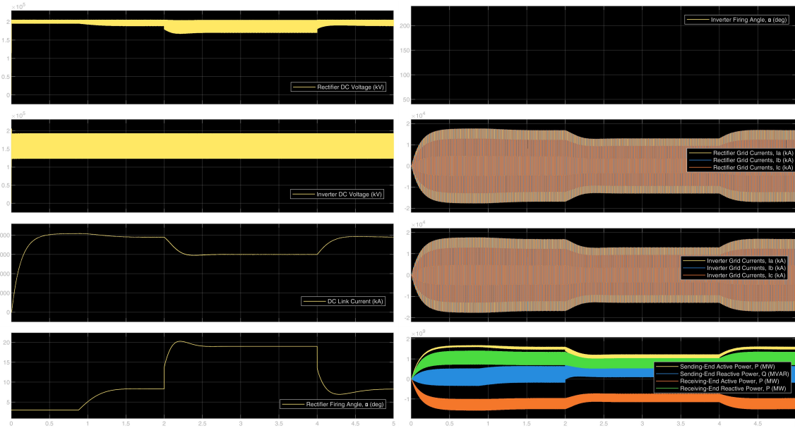
Figure 2: VI Scope: Displays the synchronization between voltages, currents, and firing angles as the system accurately tracks the step references under normal grid conditions.
