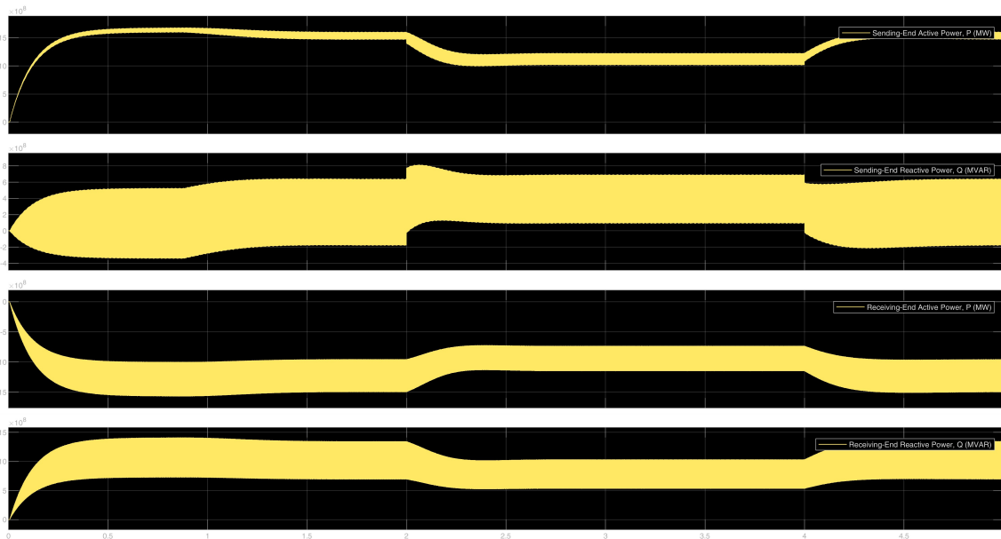
Figure 3: Powers Scope: Illustrates the corresponding active power ( P ) transmission and reactive power ( Q ) consumption profiles at both ends.
