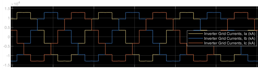
Figure 10: Inverter AC Grid Currents
