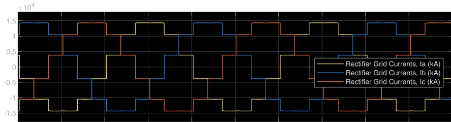
Figure 20: Rectifier Grid Currents
