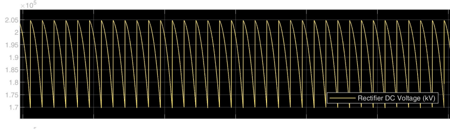
Figure 4: Rectifier DC Voltage ( V_{rect} )
