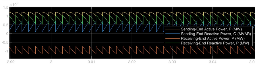
Figure 11: Active and Reactive Power ( P&Q )
