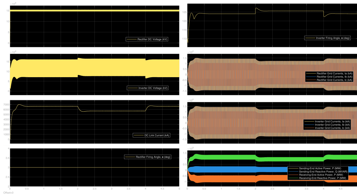
Figure 13: VI Scope: Highlights the critical transition point where the inverter abandons CEA mode and successfully takes over the Constant Current (CC) regulation.
