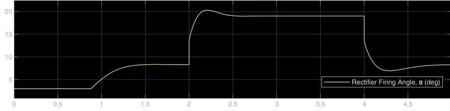
Figure 7: Rectifier Firing Angle ( \alpha_{rect} )
