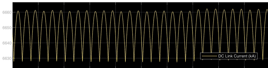
Figure 17: DC Link Current ( I_{dc} )
