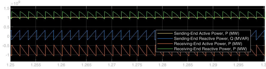
Figure 22: Active and Reactive Power ( P&Q )
